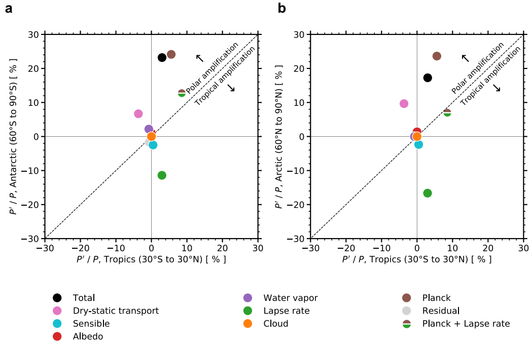
Supplemental Figure 2: Contributions to the polar amplification of relative precipitation change. Area-averaged multi-model mean relative precipitation change from 30^{\text{y}}\text{S} to 30^{\text{y}}\text{N} plotted against the area-averaged multi-model mean relative precipitation change from (a) 90^{\text{y}}\text{S} to 60^{\text{y}}\text{S} and (b) 60^{\text{y}}\text{N} to 90^{\text{y}}\text{N} . The black dot represents the total change and each colored dot represents an individual mechanism from Eq. (2) for each region in CMIP6. Changes are computed as the difference between years 130 – 150 and years 1 – 20 in abrupt-4xCO 2 simulations.
