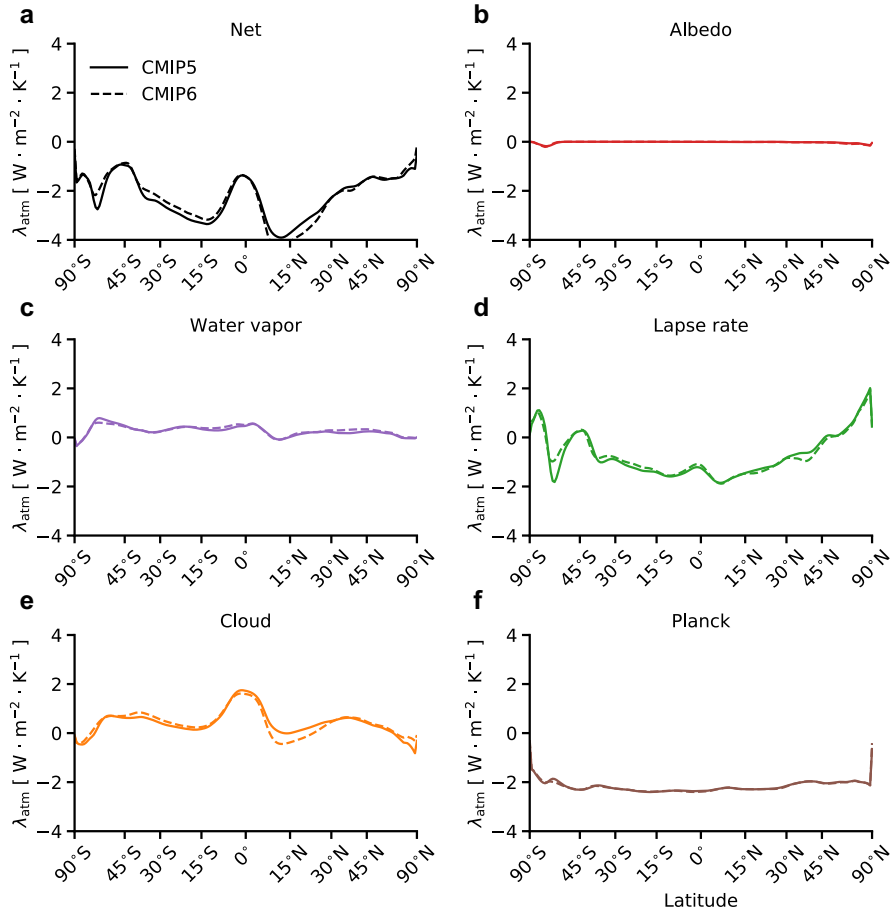
Supplemental Figure 1: Zonal-mean local atmospheric radiative feedbacks in CMIP5 and CMIP6. The zonal-mean and multi-model mean (a) total, (b) surface-albedo, (c) water vapor, (d) lapse rate, (e) cloud, and (f) Planck atmospheric radiative feedbacks for CMIP5 (solid line) and CMIP6 (dashed line). Each feedback is normalized by the local temperature change and calculated as the difference between top-of-atmosphere and surface radiative feedbacks.
